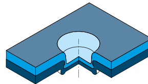
Clinchvariante R-DF, rundes Clinchelement Clinching variant R-DF, round clinching element
