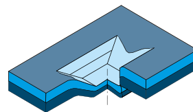
Clinchvariante S-DF, balkenförmiges Clinchelement Clinching variant S-DF, beam shape clinching element
