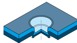
Clinchvariante G-DF, rundes Clinchelement Clinching variant G-DF, round clinching element
