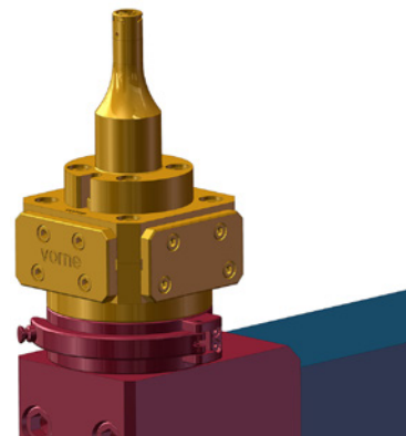
Clinchvariante G-DF, rundes Clinchelement Clinching variant G-DF, round clinching element
