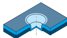
Clinchvariante CONFIX-Fügen, rundes Clinchelement Clinching variant CONFIX joining, round clinching element
