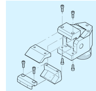
Insert mounting
