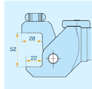
Throat
